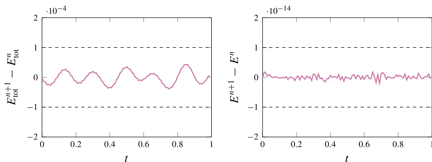
Fig. 4 Discrete total energy (80) increments (left) and generalized energy function (74) increments (right)
