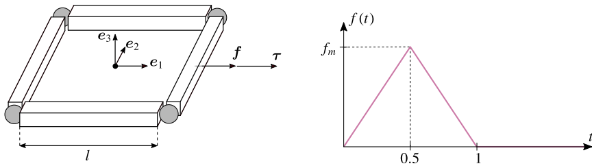
Fig. 14 Closed loop multibody system sketch (left) and temporal function of external loads (right)
